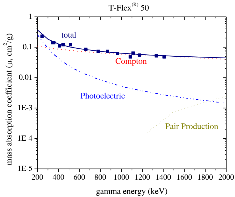
Figure 1c. Attenuation of gamma radiation T-Flex (R) 50. Measured values (squares). XCOM calculated values (lines)
