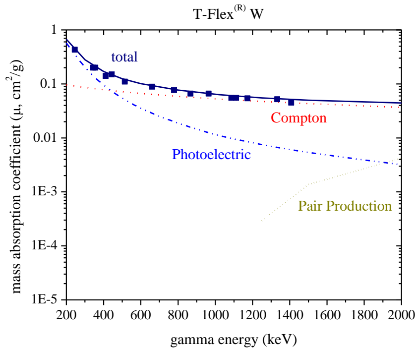
Figure 1b. Attenuation of gamma radiation T-Flex ® W. Measured values (squares). XCOM calculated values (lines)
