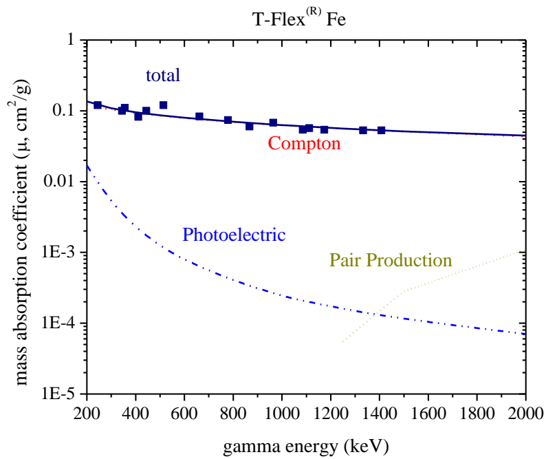
Figure 1d. Attenuation of gamma radiation T-Flex (R) Fe. Measured values (squares). XCOM calculated values (lines)
