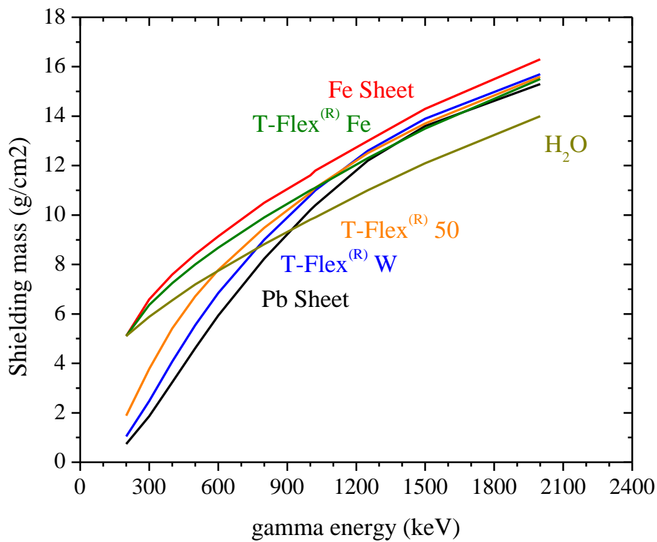
Figure 6. Mass of shielding per surface area ( \text{g}/\text{cm}^2 ) required to achieve 50% attenuation versus gamma radiation energy for selected shielding types.
